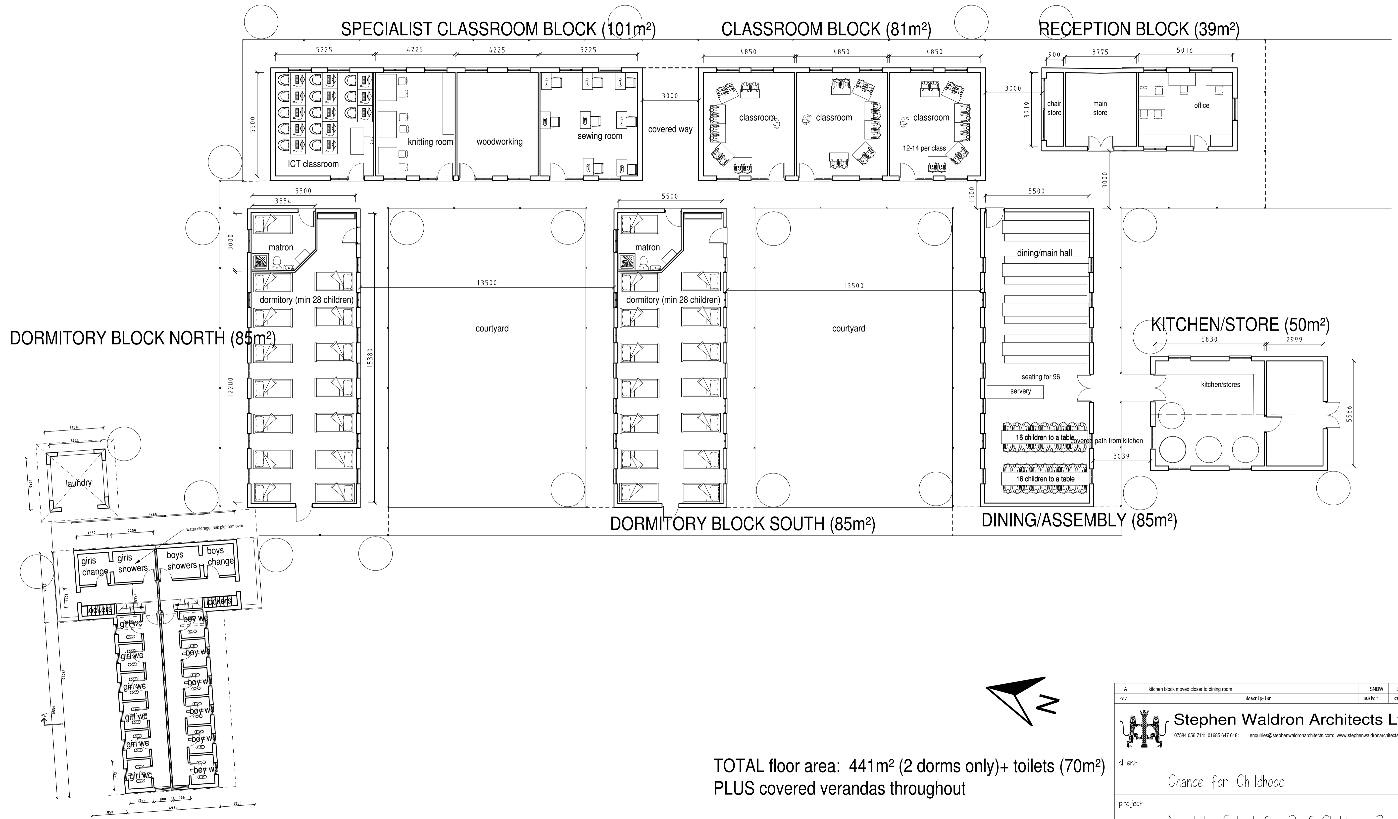
COMPOSTING TOILET/SHOWER BLOCK (70m 2 )
